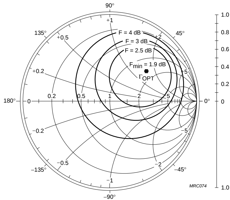
Fig.13 Noise circle.
